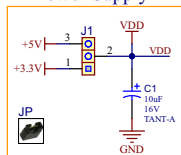
Power Supply
