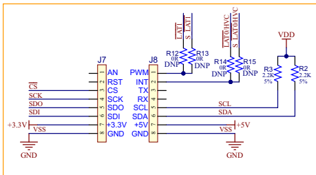
MikroBUS Connector
