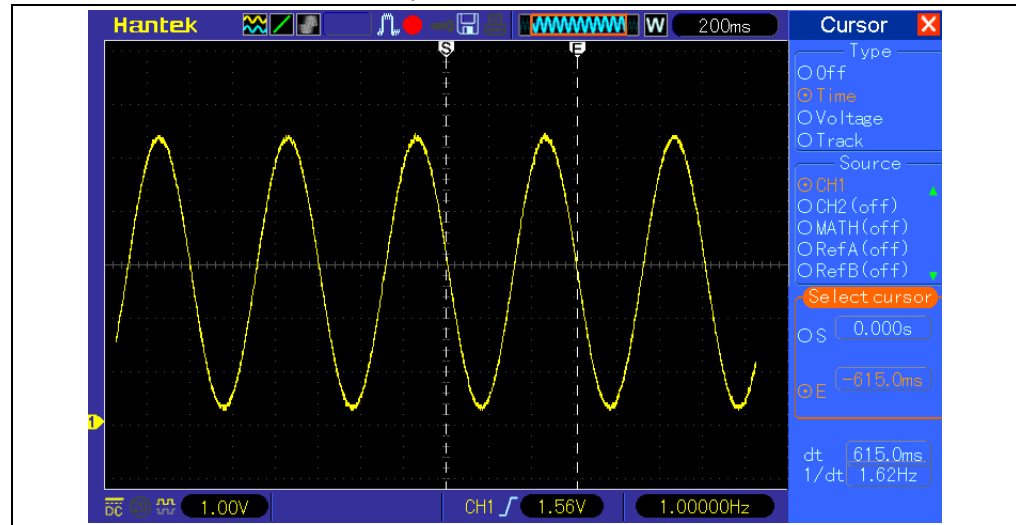
FIGURE 2-15: SPI OUTPUT SINE WAVE (LED D4 BLINKING, LEDS D2, D3 AND D5 OFF)
