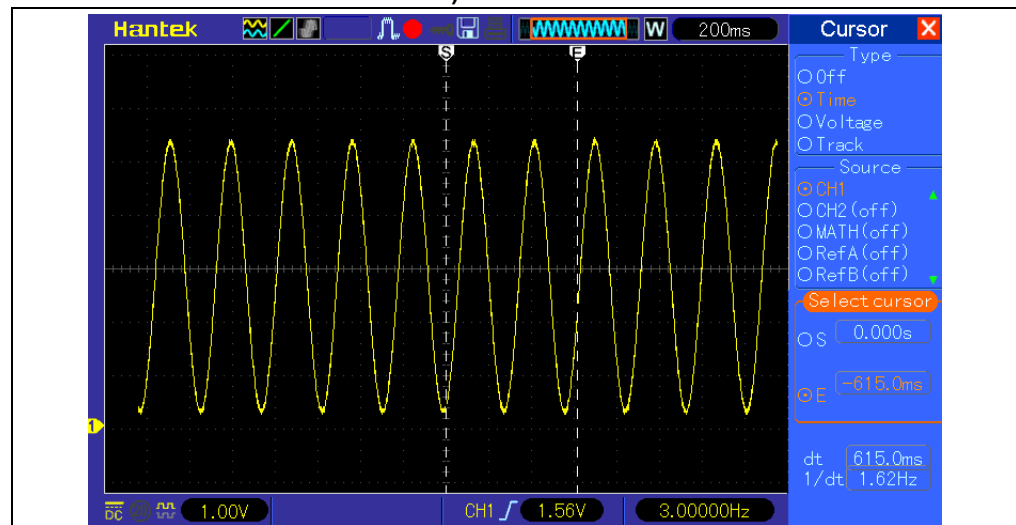
FIGURE 2-16: SPI OUTPUT SINE WAVE WITH VARYING FREQUENCY USING THE POTENTIOMETER (LED D4 BLINKING, LEDS D2, D3 AND D5 OFF)
